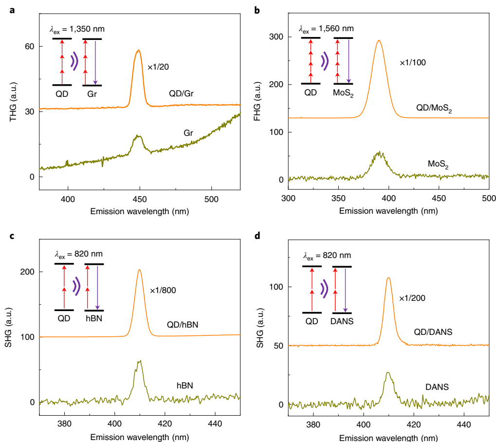
Fig. 4 | Universal optical nonlinearity enhancement of various 2D systems with different frequency harmonic orders. a, b , Enhancement of high-order frequency harmonic generations. After QD coating, both the THG of conducting graphene under excitation at 1,350 nm ( a ) and the FHG of semiconducting MoS 2 under excitation at 1,560 nm ( b ) are enhanced. Gr, graphene. c, d , Optical nonlinearity enhancement of various 2D systems. Beside conducting graphene and semiconducting MoS 2 , QD coating can also enhance the SHG of insulating hBN ( c ) and DANS ( d ) thin molecular films. The excitation wavelength for SHG is 820 nm. The insets schematically illustrate the multiphoton-excitation resonance energy transfer from the QDs to the 2D materials for optical nonlinearity enhancement.
