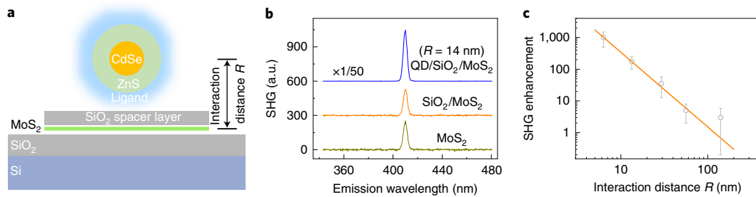
Fig. 2 | Interaction-distance-dependent SHG enhancement. a , Schematic illustration of the fabricated QD/SiO 2 /MoS 2 sandwich hybrid structure by sequentially depositing SiO 2 and QDs on MoS 2 . The interaction distance R between MoS 2 and the QD film can be systematically tuned by the thickness of the SiO 2 spacer layer. b , SHG spectra of MoS 2 and the fabricated hybrid structures. With an interaction distance of ~14 nm, the SHG intensity of MoS 2 can still be enhanced by ~170 times. For comparison, without QDs, the SiO 2 layer hardly influences the SHG intensity. c , Interaction-distance-dependent SHG enhancement. Increasing the interlayer distance quickly weakens the SHG enhancement, with a fitted power coefficient of -2.3 . Error bars are the standard deviation measured from ten samples.
