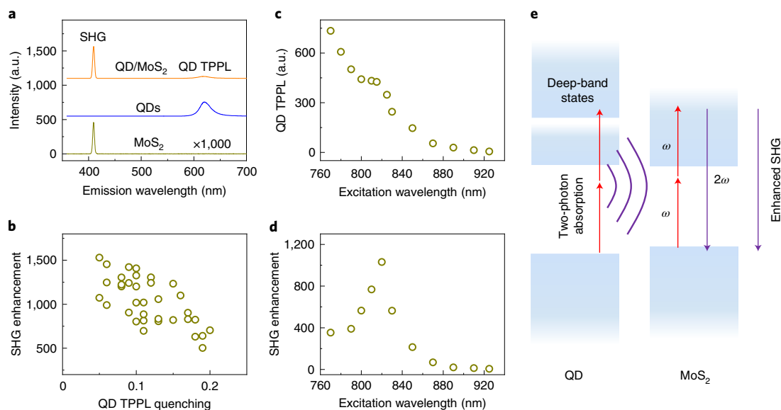
Fig. 3 | Excitation-wavelength-dependent SHG enhancement. a , SHG and TPPL spectra of the pristine MoS 2 monolayer, QD film and their hybrid under 820 nm pulsed-laser excitation. The sharp peak at 410 nm is the SHG of MoS 2 and the broader peak at 620 nm corresponds to the TPPL of the QDs. Compared with its component layers, the QD/MoS 2 hybrid shows an enhanced MoS 2 SHG and a quenched QD TPPL. b , The MoS 2 SHG enhancement versus QD TPPL quenching in the hybrid structure obtained from around 40 samples. When the SHG was enhanced more noticeably, the QD TPPL was quenched more significantly. c,d , Wavelength-dependent TPPL of the pristine QD film ( c ) and SHG enhancement in the QD/MoS 2 hybrid ( d ) under two-photon excitation. The TPPL spectrum of the QDs presents a shoulder around ~820 nm, indicating the existence of deep-band excited states with a strong oscillator strength and high two-photon absorption. By coincidence, the SHG enhancement in the hybrid shows a peak at ~820 nm as well. e , Scheme of multiphoton-excitation resonance energy transfer and SHG enhancement. Under resonant excitation of the deep-band two-photon excited states in the QDs, strong dipole coupling and perfect energy overlap between the QDs and MoS 2 facilitate the high-efficiency energy transfer and hence substantially strengthen the second harmonic response.
