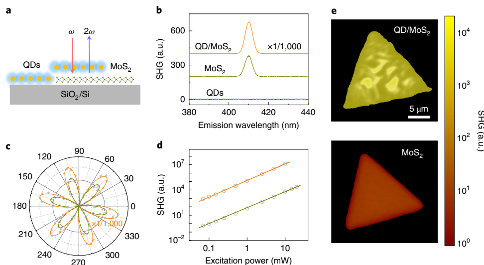
Fig. 1 | MoS 2 monolayer SHG enhancement with QD coating. a , Side-view illustration of the QD/MoS 2 hybrid structure and its optical SHG. b , SHG spectra of MoS 2 and QD/MoS 2 under 820 nm pulsed-laser excitation. With a QD coating, the weak SHG of MoS 2 can be boosted by \sim 1,500 times in the hybrid. For comparison, no apparent SHG signal can be observed for the pristine QDs. c , Polarization-dependent SHG patterns measured on a MoS 2 monolayer (dark yellow) and its QD hybrid (orange). d , Excitation power dependence of the SHG peak intensity for MoS 2 (dark yellow) and the QD/MoS 2 hybrid (orange), where both curves show the expected quadratic law. e , Spatial SHG intensity mapping images of a MoS 2 monolayer before (lower) and after (upper) QD coating.
