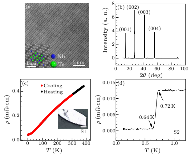
Fig. 1. Characterization and \rho - T behavior of NbTe 2 . (a) The HAADF-STEM image of NbTe 2 viewed from [010] direction, where the scale bar represents 5 nm. Inset is the enlarged view of the HAADF image overlaid with the atomistic model. Blue balls: Nb; green balls: Te; scale bar: 1 nm. (b) XRD of (00 l ) surface of single crystal NbTe 2 . Labels assign peaks to the corresponding crystalline surfaces. (c) Resistivity as a function of temperature of NbTe 2 down to 2 K. Red and black curves indicate the data obtained during cooling and heating process. No signal of structural phase transition is observed. Inset is an optical picture of the NbTe 2 sample, where the scale bar represents 0.5 mm. (d) SC transition in \rho - T behavior. Labels indicate zero and onset transition temperature.
