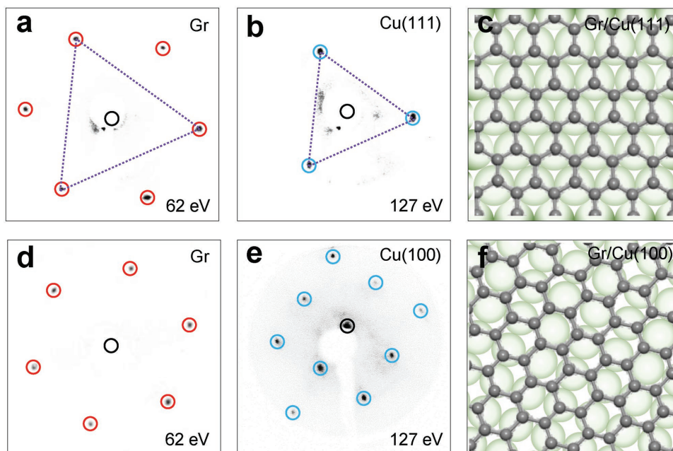
Figure 2. Reciprocal-space surface configuration in Gr/Cu systems. a,b) LEED patterns of graphene and the Cu(111) underneath obtained under different electron energies. The identical crystalline direction of graphene and Cu(111) demonstrates the epitaxial graphene growth. c) Schematic diagram of graphene lattice on Cu(111). Carbon atoms are well matched with Cu. d,e) LEED patterns of graphene and the Cu(100) underneath obtained under different electron energies. Graphene lattice shows a twist angle with Cu(100). f) Schematic diagram of graphene lattice on Cu(100). Carbon atoms cannot match with Cu. Gray (green) balls denote carbon (Cu) atoms in (c) and (f).
